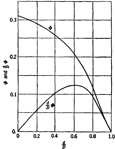
FIG. 15-7.—Parameter \phi as a function of d/D .
